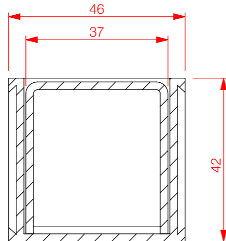
SECTION Q-Q SCALE 1 : 1
