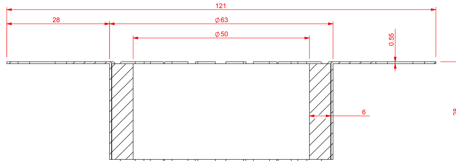
SECTION
