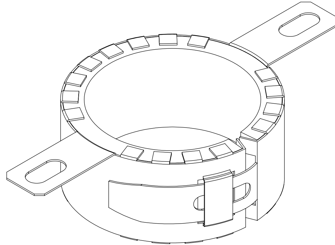
ISOMETRIC VIEW
